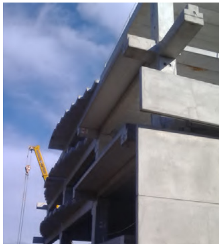
» STRATOS multi-storey structure with overhangs and panels.
