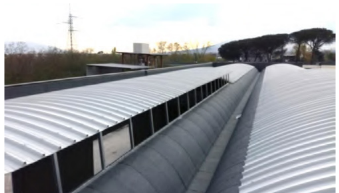
» Roofing between 'PRISMA' elements with Sandwich Panel - External view
